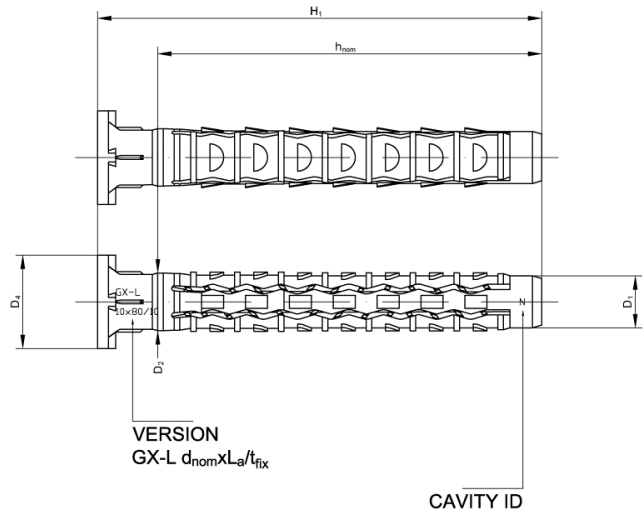
Version with collar for size \phi 10 only
